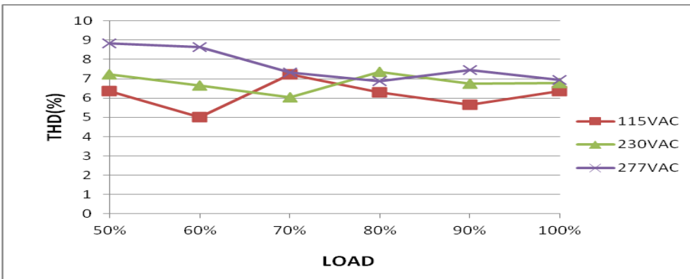
THD&LOAD
